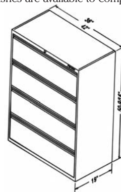
1204-36 (4) DRAWER UNIT 36" WIDE 1204-42 (4) DRAWER UNIT 42" WIDE
